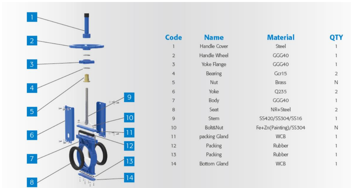
Exploded View Of Rubber Sealed Knife Gate Valve
