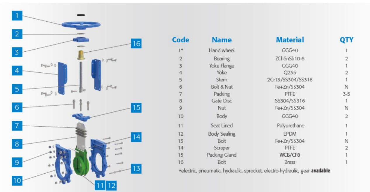
Exploded View Of PU Seated Knife Gate Valve
